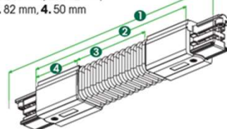
Adjustable corner connector XTS 24 1. 226 mm, 2. 160 mm, 3. 60 mm, 4. 50 mm
