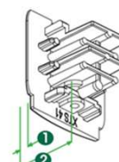
End cap XTS-41 1. 3 mm, 2. 21 mm
