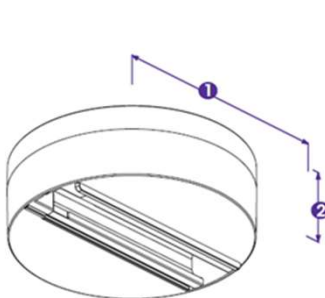
GA 70 1. 100 mm 2. 32 mm
